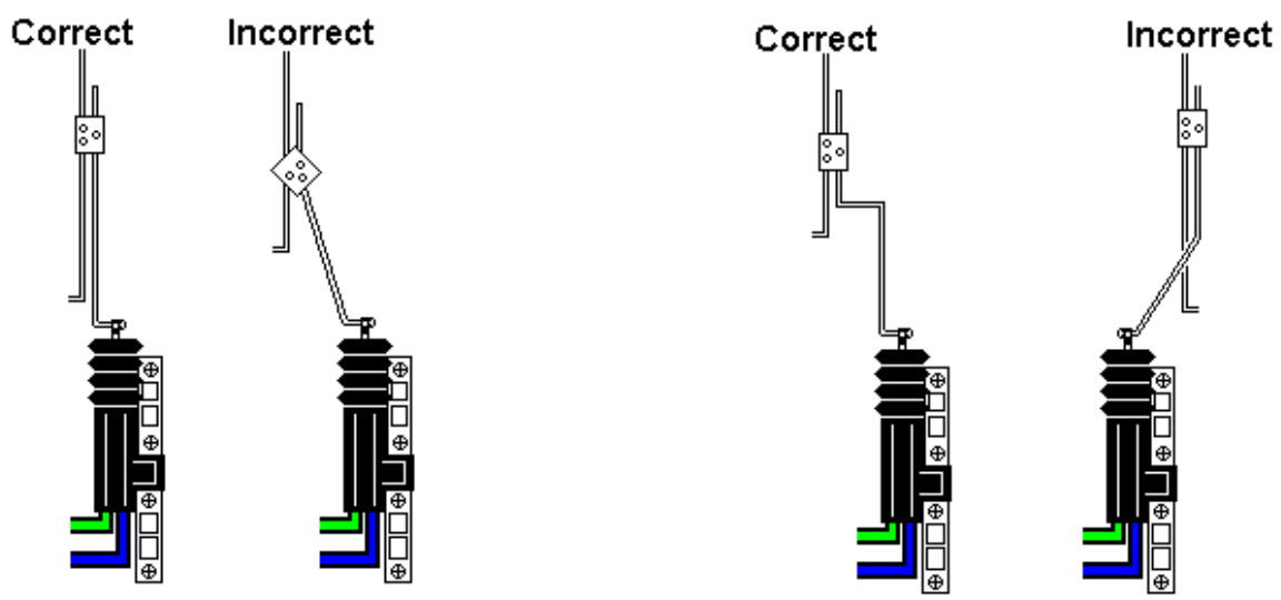
Fig. 2 Actuators CANNOT be INSTALLED in a bind
