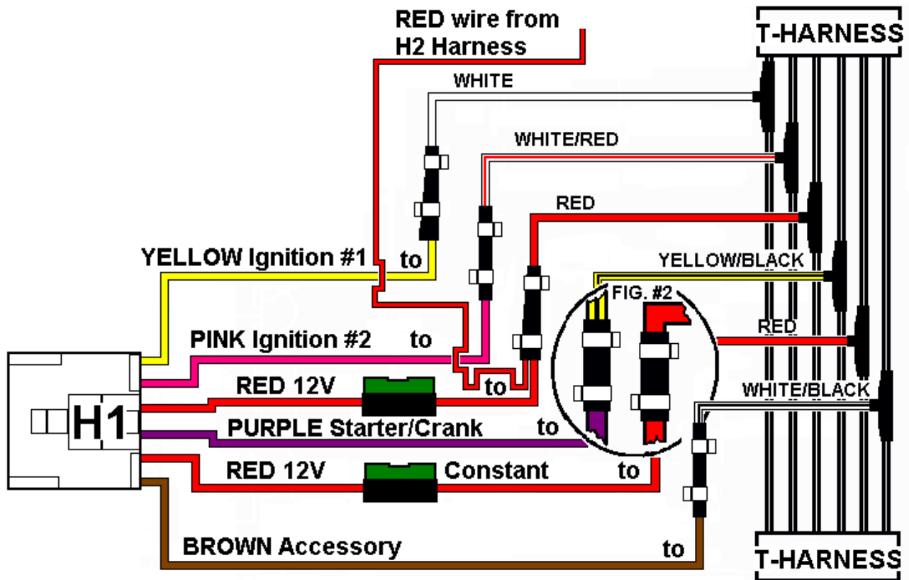
FIG. #2 Shows the connection between the T-Harness outgoing connectors and the H1 Harness from the unit. Note ** this is an END to END connection.
