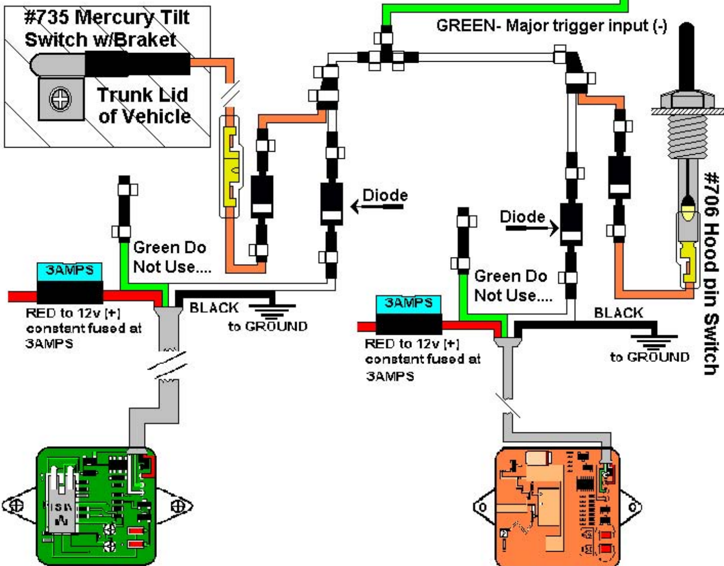
#700 SHOCK SENSOR
